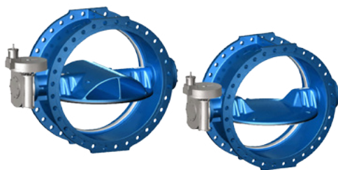
Flow-through disc
